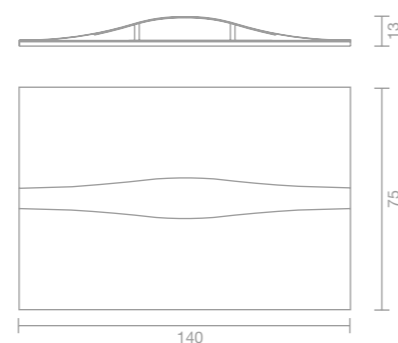
ART. 4501 Applique / Wall lamp Applique / Wandleuchte 140 cm - 55''12 H.75 cm - H.29''53 1x55W - 2G11 -
